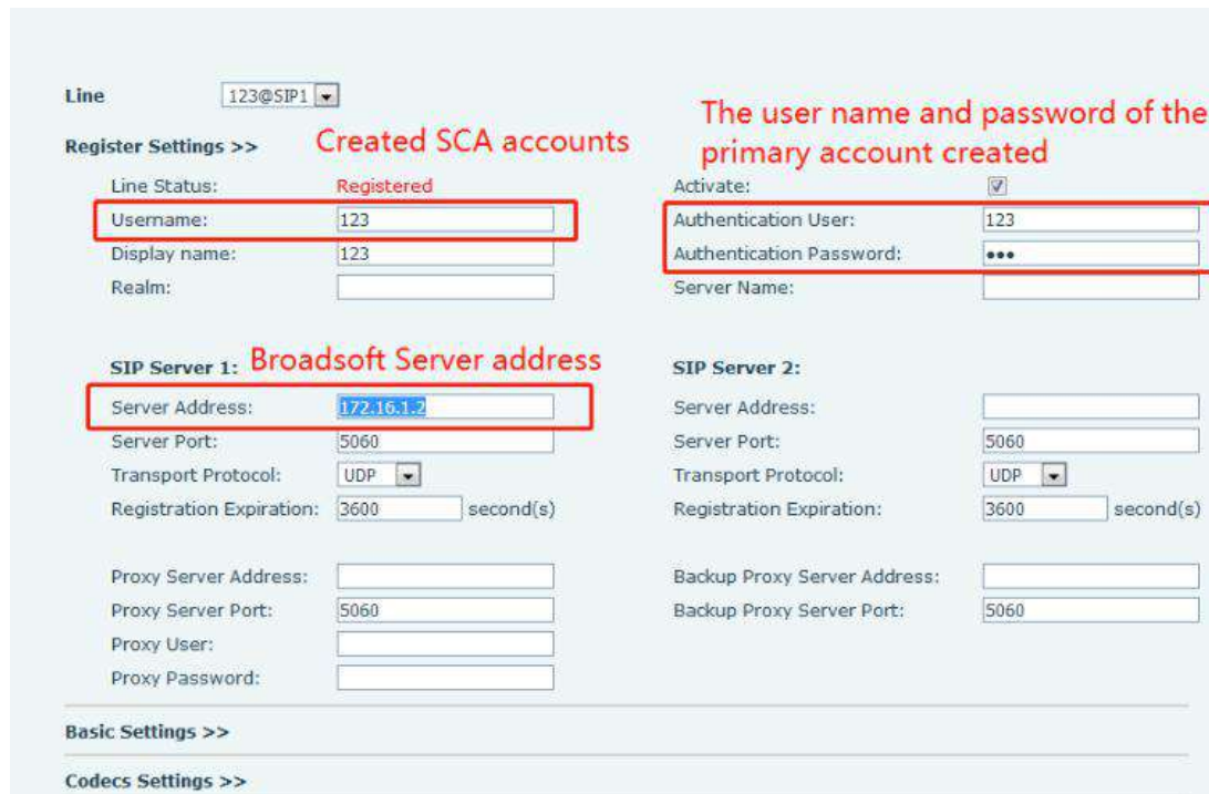
Picture 75 - Register BroadSoft account
