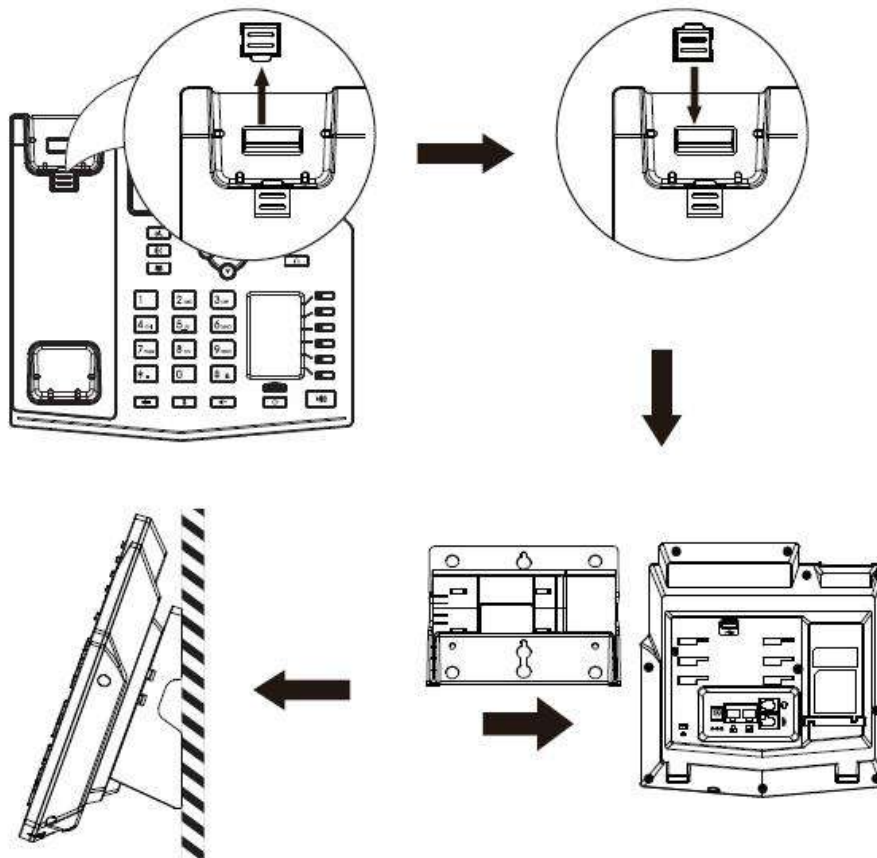
Picture 2 - Wall-mounted installation
