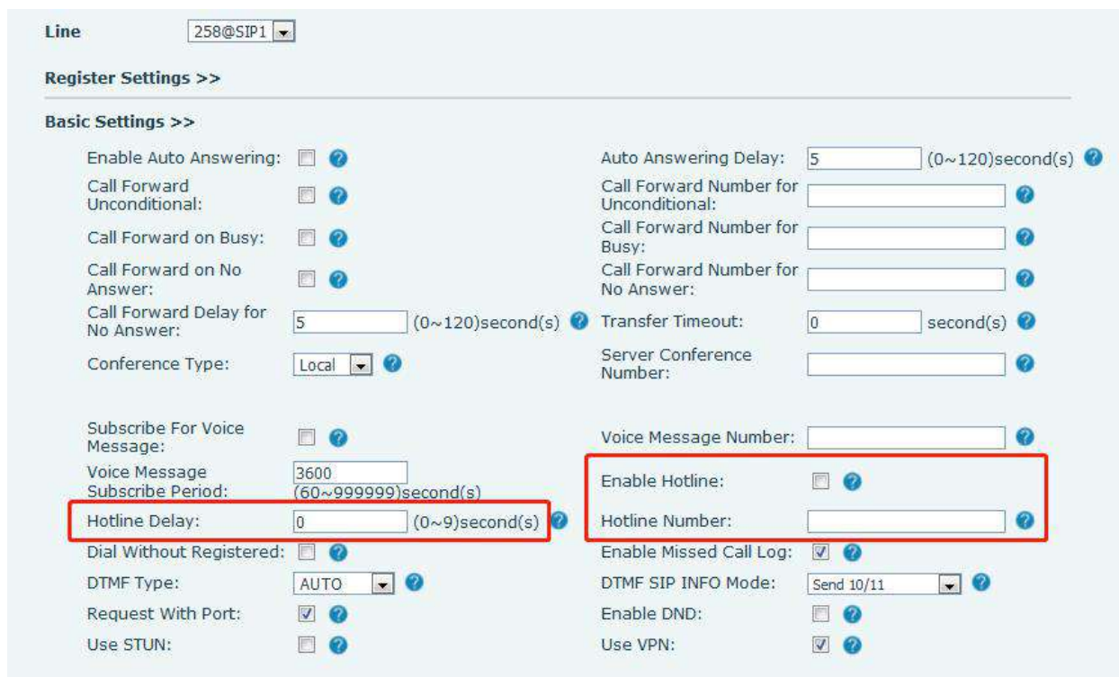
Picture 60 - Hotline set up on webpage
