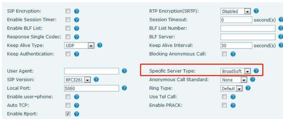
Picture 76 - Set BroadSoft server
